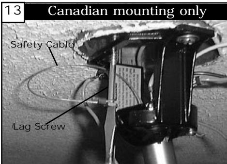
13 Canadian mounting only Safety Cable Lag Screw For Canadian installation in both flush and downrod mode the safety cable must be installed into the house structure beams using the 3" lag screws provided. Make sure that when the safety cable is fully extended the leadwires are longer than the cable and no stress is placed on the leadwires.
